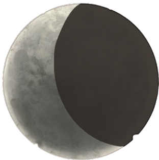
Shadows cast by the Earth on the Moon during a lunar eclipse.
