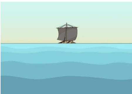
Observations of ships sailing across the horizon.
